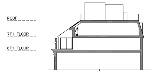
04 PROPOSED SECTION Scale: 1:200
