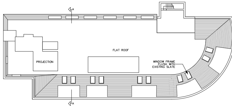
03 PROPOSED ROOF PLAN Scale: 1:200
