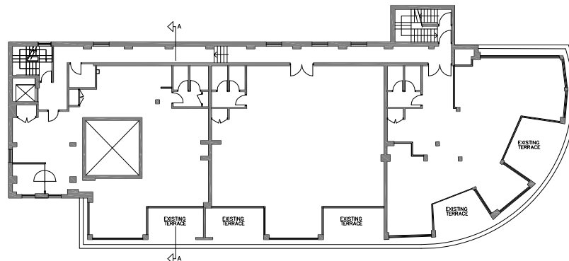
01 PROPOSED 6TH FLOOR PLAN Scale: 1:200
